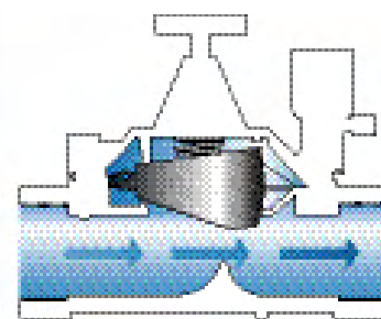
The UltraFlow Series straight-through flow path
